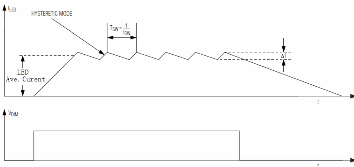
Figure 4 Current Regulation
