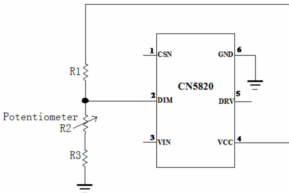
Figure 3 Analog Dimming by Using a Potentiometer
